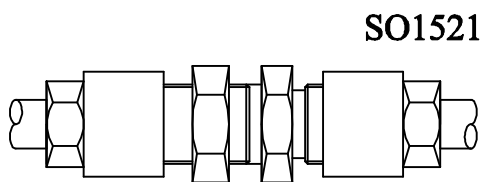
SO1521 Panel mount union (max. panel thickness 5mm). Raccordo passaparete (spessore max. parete 5mm)
