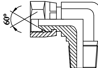
Elbow adaptors Adattatori a gomito
