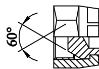
Plugs female Tappi femmina
