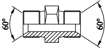
Straight adaptors Nippli
