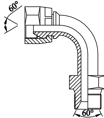
Elbow adaptors Adattatori a gomito
