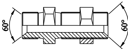
Bulkhead adaptors
